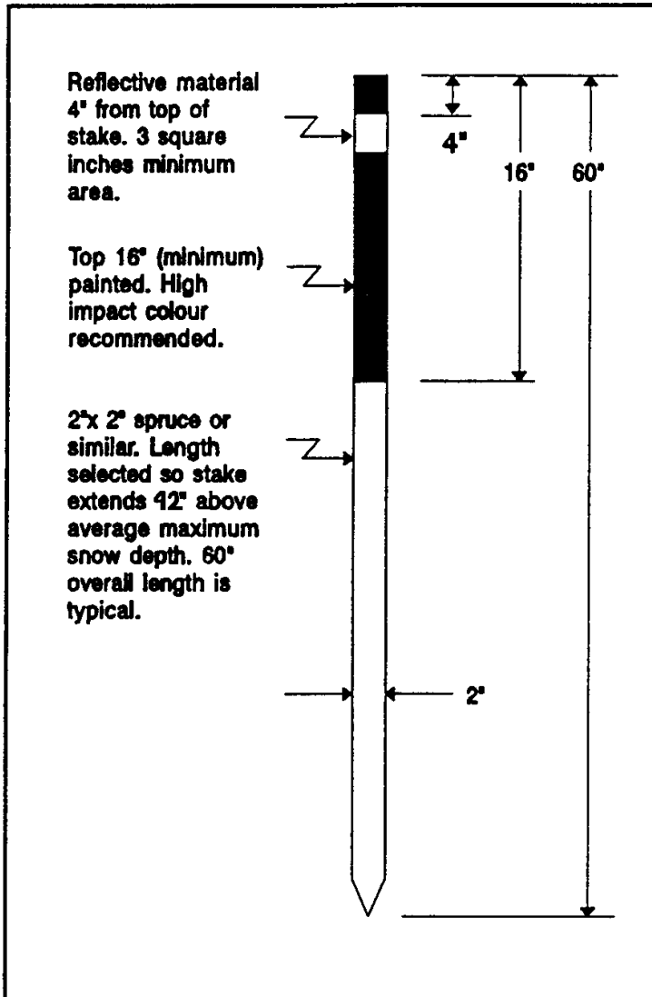
Figure 4 - Recommended Stake
